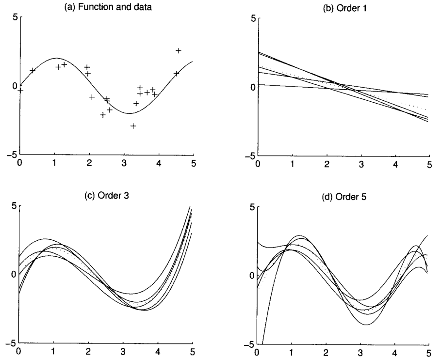
Figure 4.5 (a) Function, f(x) = 2 \sin(1.5x) , and one noisy ( \mathcal{N}(0,1) ) dataset sampled from the function. Five samples are taken, each containing twenty instances. (b), (c), (d) are five polynomial fits, namely, g_i(\cdot) , of order 1, 3, and 5. For each case, dotted line is the average of the five fits, namely, \bar{g}(\cdot) .
